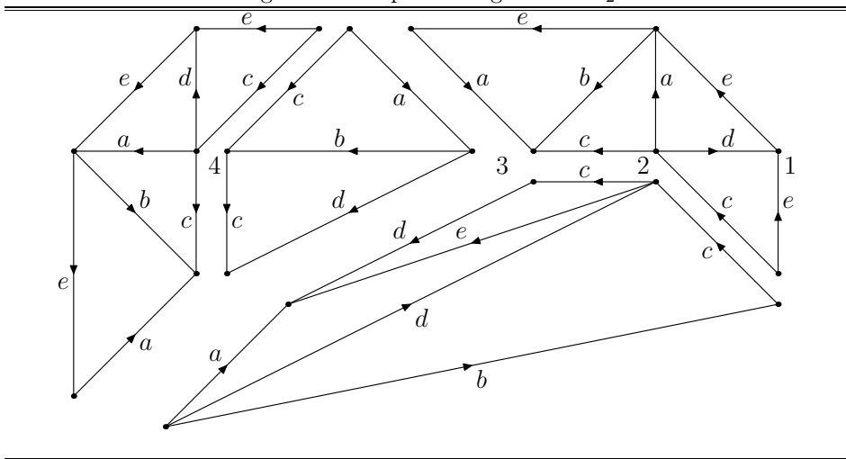
Figure 3. Composite diagram for \Psi_2
