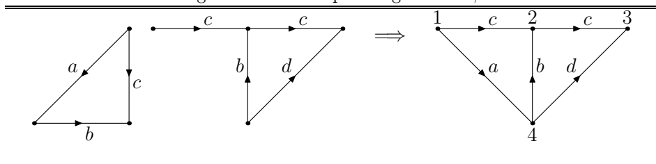
Figure 2. van Kampen diagram for c\beta
