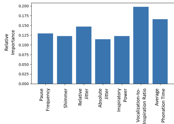
Fig. 5. Feature Importance
