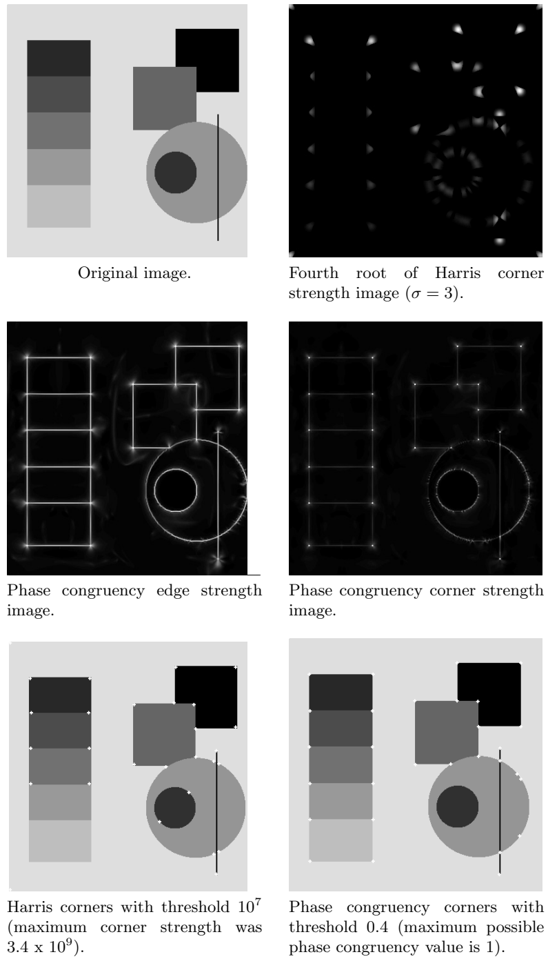
Fig. 3. Comparison of the Harris and phase congruency operators on a test image.
