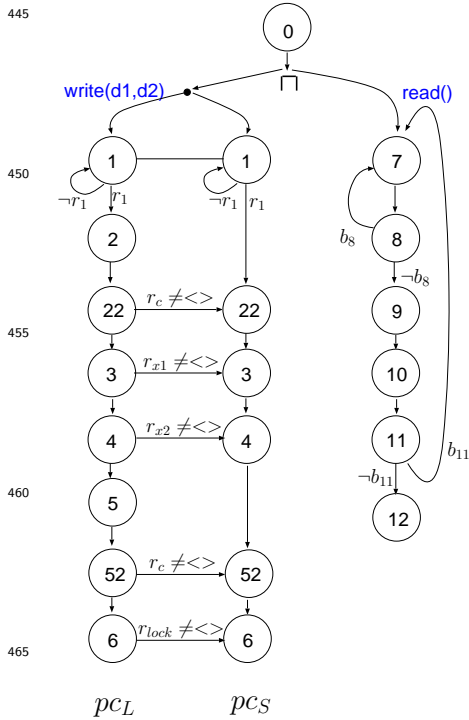
Figure 6: A flow graph of the seqlock under TSO
